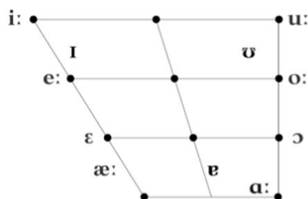
Figure 2. The IPA symbols used for the pure vowels of Standard Lithuanian
